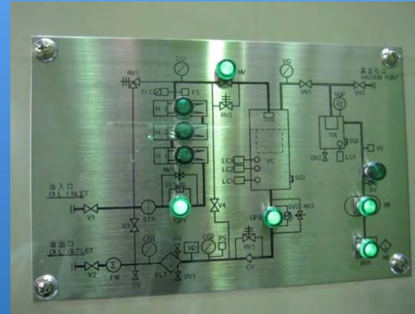
MIMIC GRAPHIC: Monitor operation
